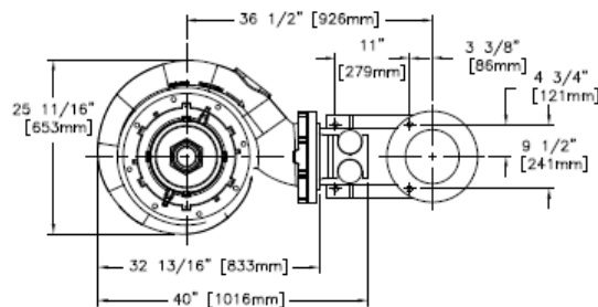
SECTION B-B
